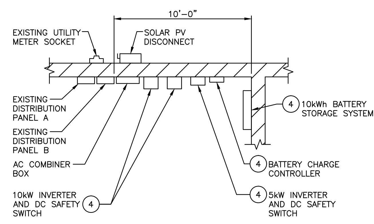
EQUIPMENT LAYOUT 0 1' 2' 4' 8'
